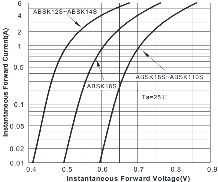
FIG3: Forward Voltage
